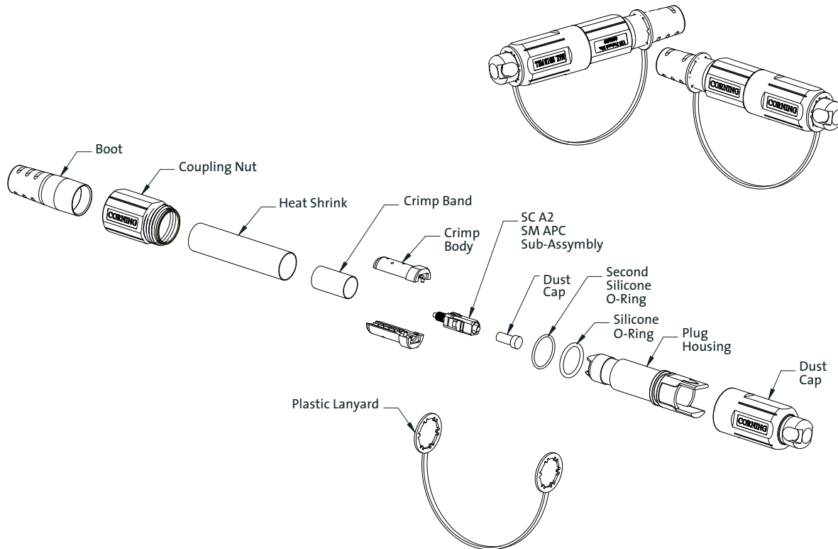
OptiTap® SC Plug Connector Assembly, Flat Drop | Drawing ZA-2918
